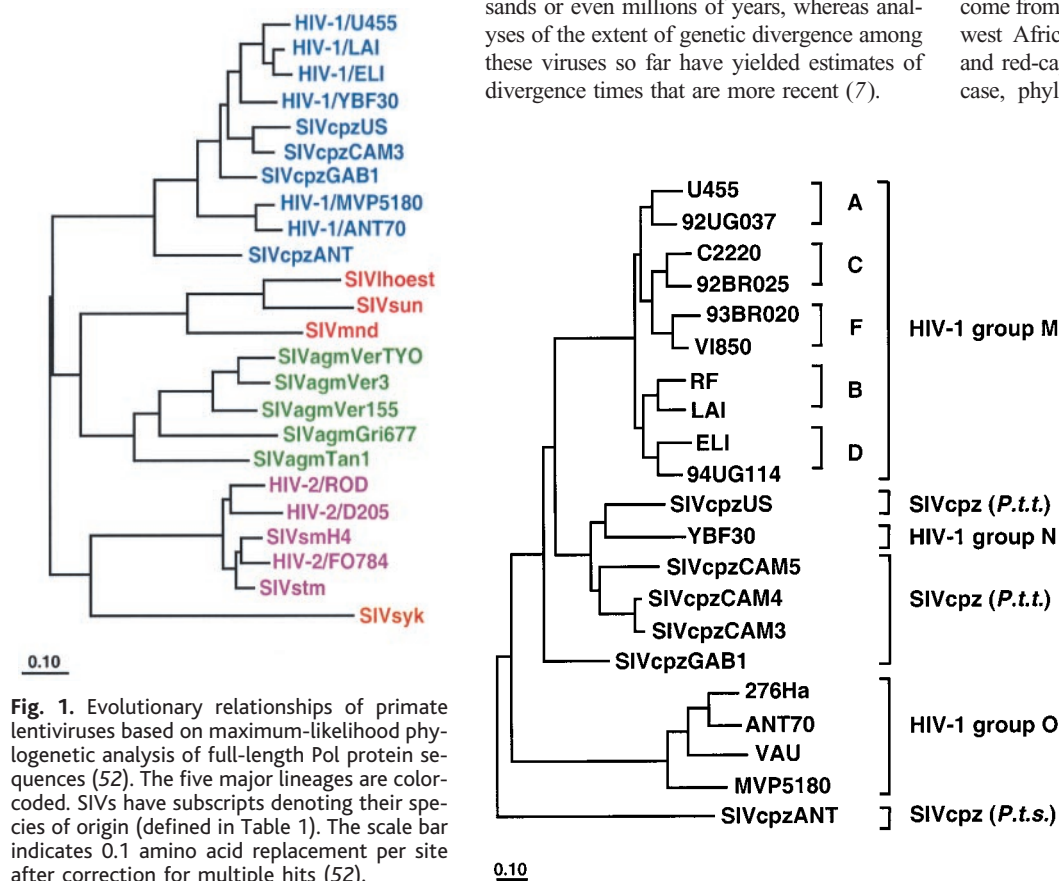
Fig. 2. Evolutionary relationships of members of the HIV-1/SIVcpz lineage based on maximum-likelihood phylogenetic analysis of full-length Env protein sequences (52). The three groups of HIV-1 (M, N, and O) are indicated by brackets at the right, as are five representative subtypes of the M group (A through F). The SIVcpz strains were isolated from either P. t. troglodytes ( P.t.t. ) or P. t. schweinfurthii ( P.t.s. ) animals. The scale bar indicates 0.1 amino acid replacement per site after correction for multiple hits (52).
